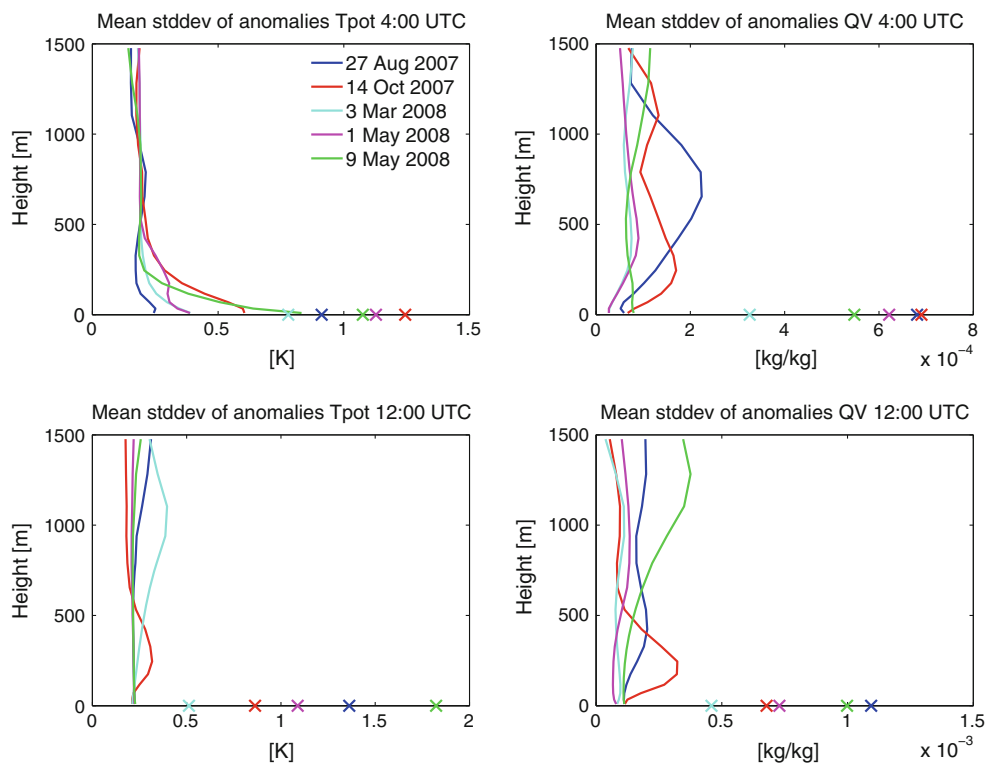
Fig. 3 Mean subgrid-scale (400 m) standard deviations per coarse pixel (2.8 km) for potential temperature ( left ) and specific humidity ( right ) for 4:00 ( top ) and 12:00 UTC ( bottom ) in the atmosphere ( lines ) and at the surface ( marked by crosses )
