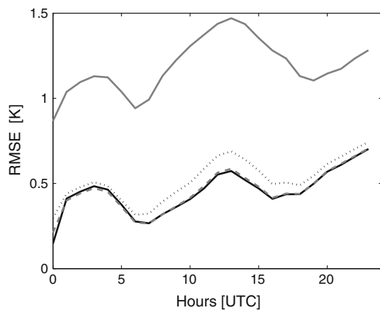
Fig. 5 Root mean square differences for the temperature difference T - T_s between lower atmosphere (lowest model level) and surface with respect to the high-resolution reference. Lines indicate the model configuration as in Fig. 4, i.e. light grey solid coarse, black solid mosaic, dashed no noise, dotted with noise
