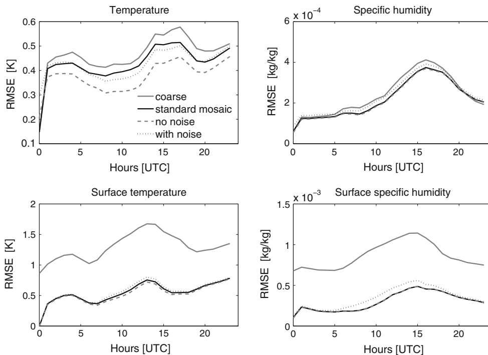
Fig. 4 Root mean square differences for atmospheric ( top ) and surface ( bottom ) temperature ( left ) and specific humidity ( right ), averaged over all case studies for the model configurations as listed in Table 3
