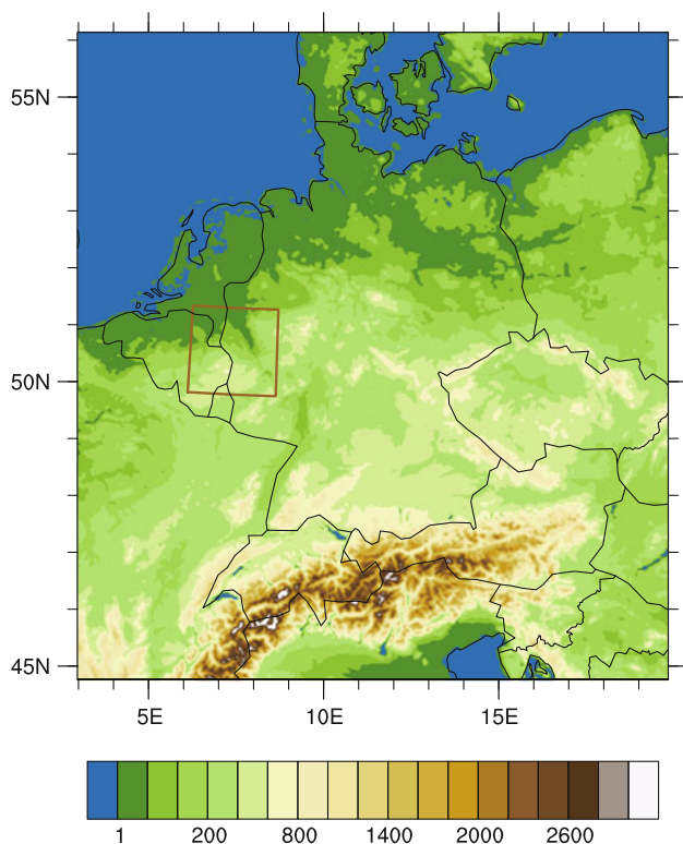
Fig. 1 Model domain of the standard COSMO-DE model configuration with 2.8-km grid spacing and the smaller model domain used for the case studies indicated by the square . The colouring indicates the orographic relief height (m)
