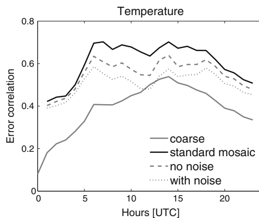
Fig. 6 Correlations of errors of surface and atmospheric temperature, averaged over six case studies
