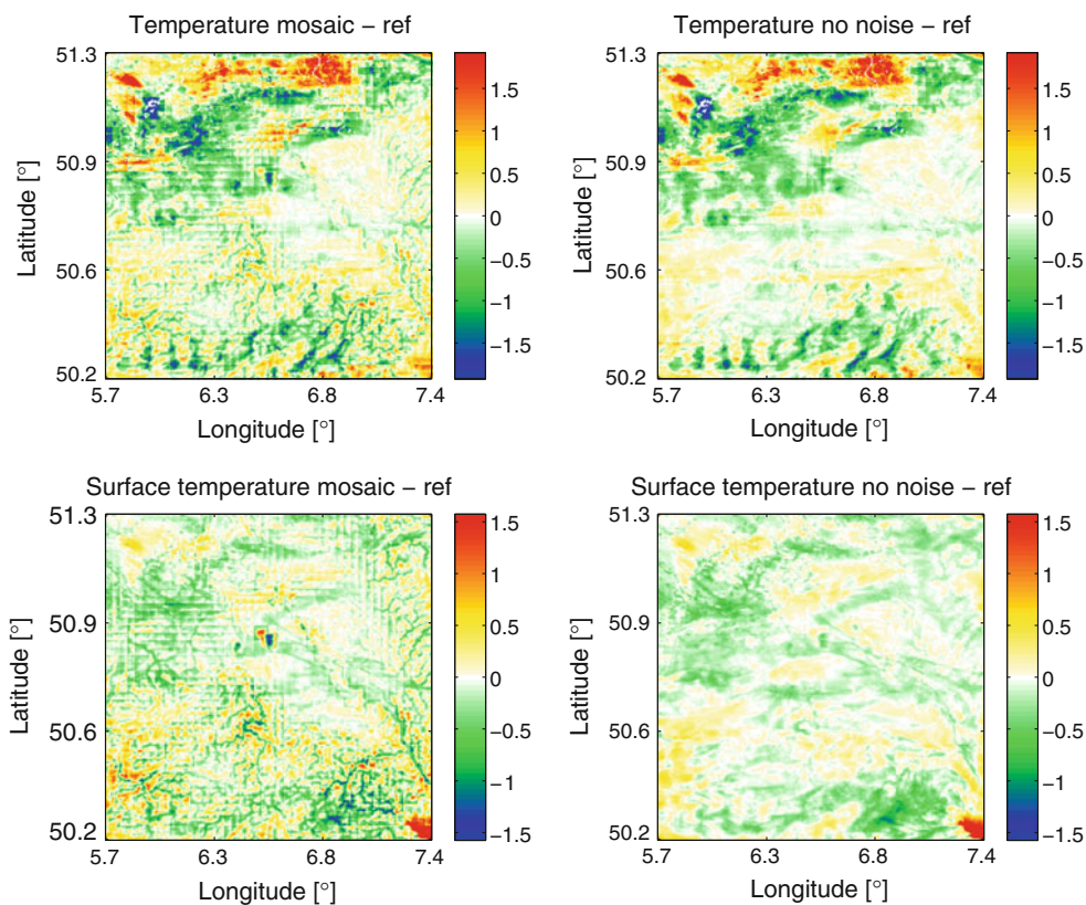
Fig. 7 Temperature (K) ( top ) and surface temperature (K) ( bottom ) difference field (with respect to the high-resolution reference) for 12:00 UTC on 16 July 2008 for model run with pure mosaic ( left ) and mosaic plus downscaling step 1 and 2 ( right )
